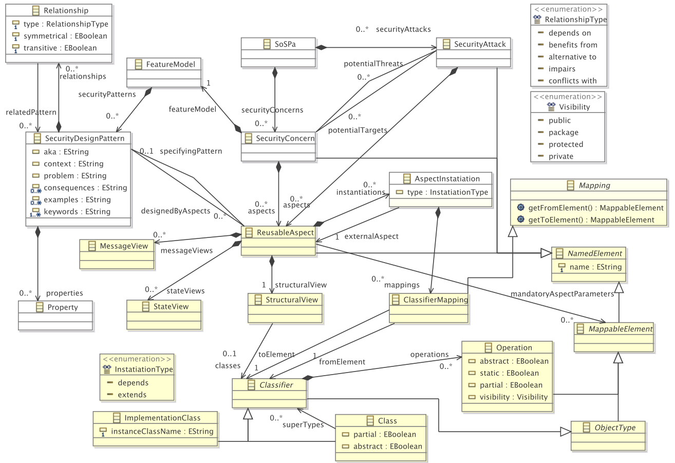
Figure 1: Meta-model of A System of aspect-oriented Security design Patterns (SoSPa-MM)
