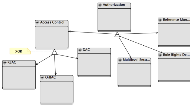
Figure 2: A Feature Model of Authorization
