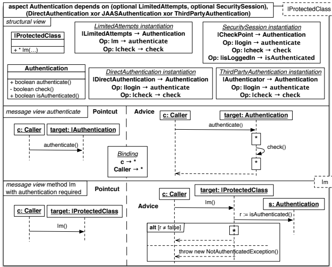
Fig. 5. Aspect Authentication
