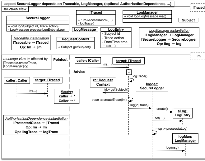
Fig. 11. Aspect SecureLogger
