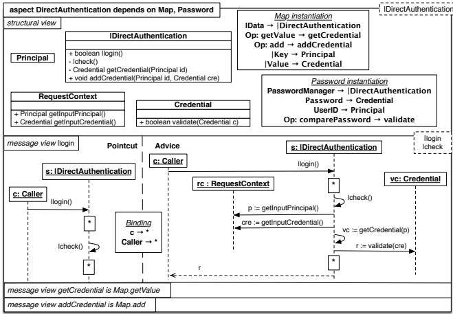
Fig. 6. Aspect DirectAuthentication
