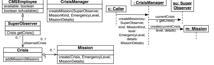
Fig. 2. A Partial Design of CMS with createMission Function [7]
