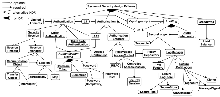
Fig. 4. A Partial Feature Model of SoSPa
