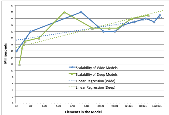
Fig. 6. Scalability of read operations for large-scale models
