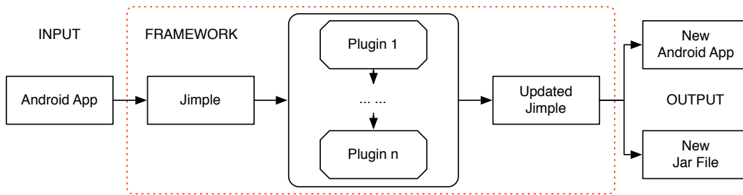
Figure 2: The work process of our generic framework.
