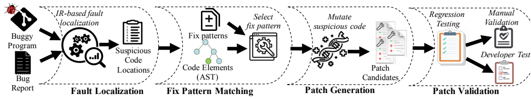
Figure 2: The iFixR Program Repair Workflow.
