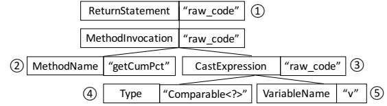
Figure 4: Buggy code of Defects4J bug Math-75.
