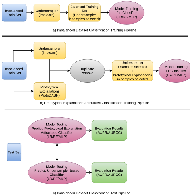
Fig. 1. Imbalanced Dataset Classification Pipeline
