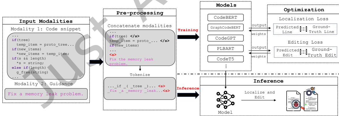
Fig. 3. Overview of our JLED pipeline.
